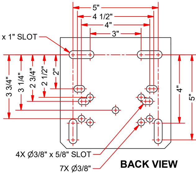
PIG TAIL NET ATTACHMENT SYSTEM (12 PLACES)
