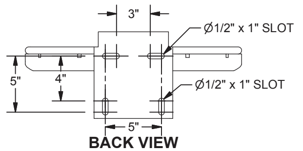
DETAIL A HIDEAWAY NET ATTACHMENT SYSTEM (12 PLACES)
