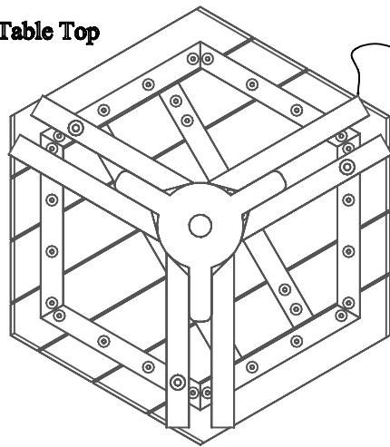
F - Small Spoke Assembly
