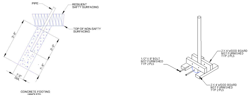
Diagram: Suggested Bracing Method
