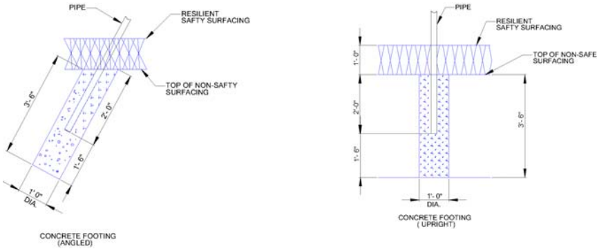
Diagram: Permanent Installation
