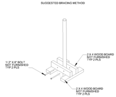
Diagram: Suggested Bracing Method
