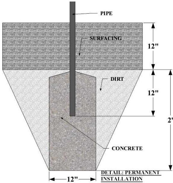
Diagram: Permanent Installation
